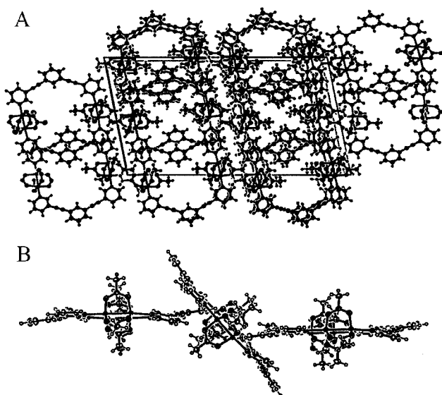
Figure 2. A: The packing in the unit cell viewed along the a axis; B: view showing the partial penetration of two complexes into a central tilted complex.
