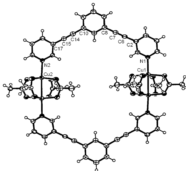
Figure 1. Ortep view of the 2:4 complex formed between 1 and copper(II) acetate; ellipsoids drawn at the 50% probability level
